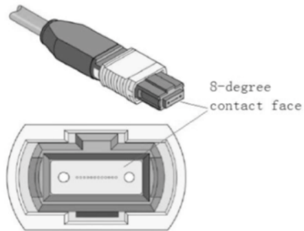
Figure 19 MTP/APC Cable
